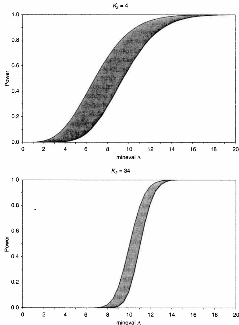
Figure 5.5. Power function for TOLS bias test (Relative bias = 0.1, n = 2 ).
