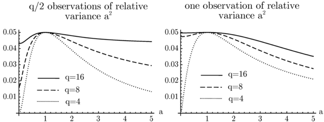
Figure 1: Null Rejection Probabilities of 5% Level t -tests with q Independent Observations
