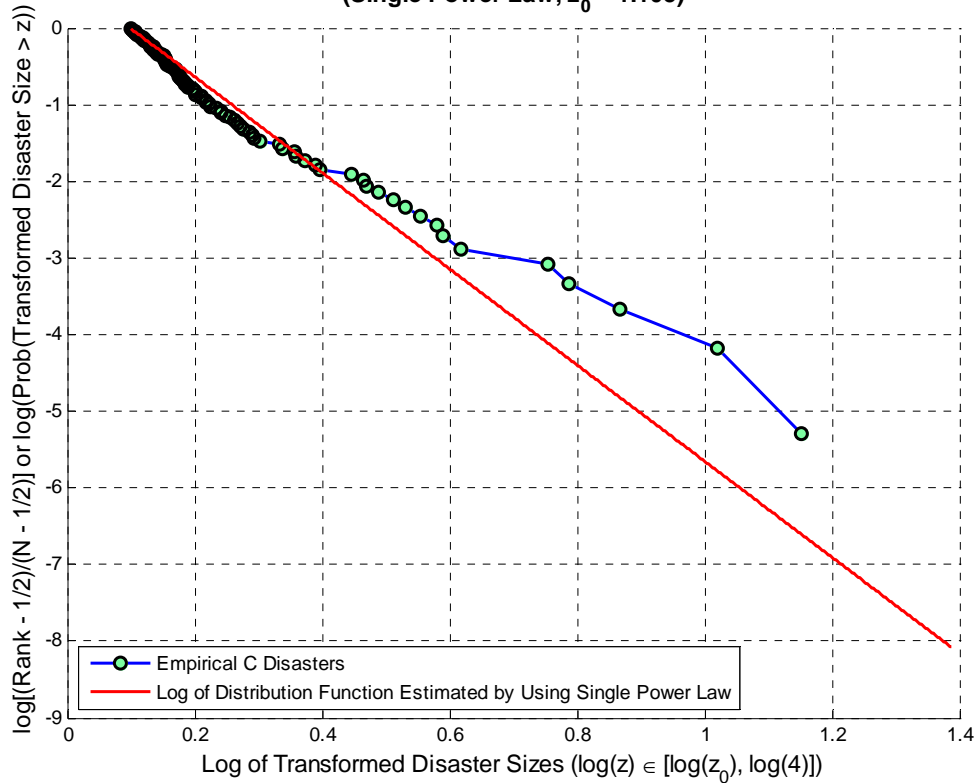
Log C Disaster Sizes vs \log[(\text{Rank} - 1/2)/(N - 1/2)] & Estimated Distribution Function (Log Scale) (Single Power Law, z_0 = 1.105 )
